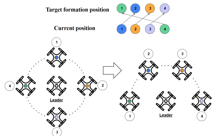
Fig. 4. Target formation position allocation optimization using Hungarian algorithm
